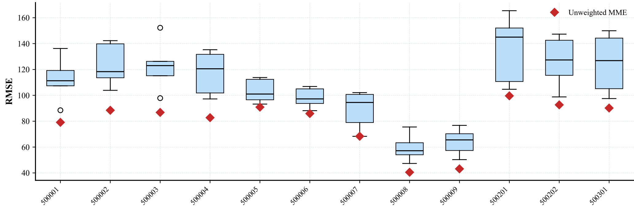
Individual-model spread versus unweighted MME — RMSE, monthly, independent validation
